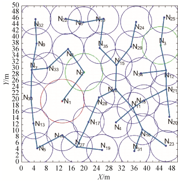
图 10 节点最终部署图 Fig. 10 Final deployment of the network
