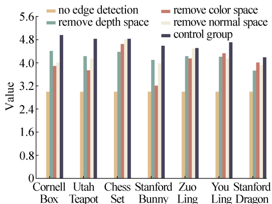
图 8 屏幕空间三相边缘检测的消融实验结果 Fig. 8 Results of ablation experiment on screen space three-phase edge detection
